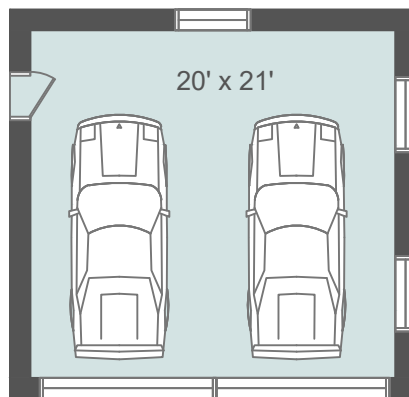
Garage
